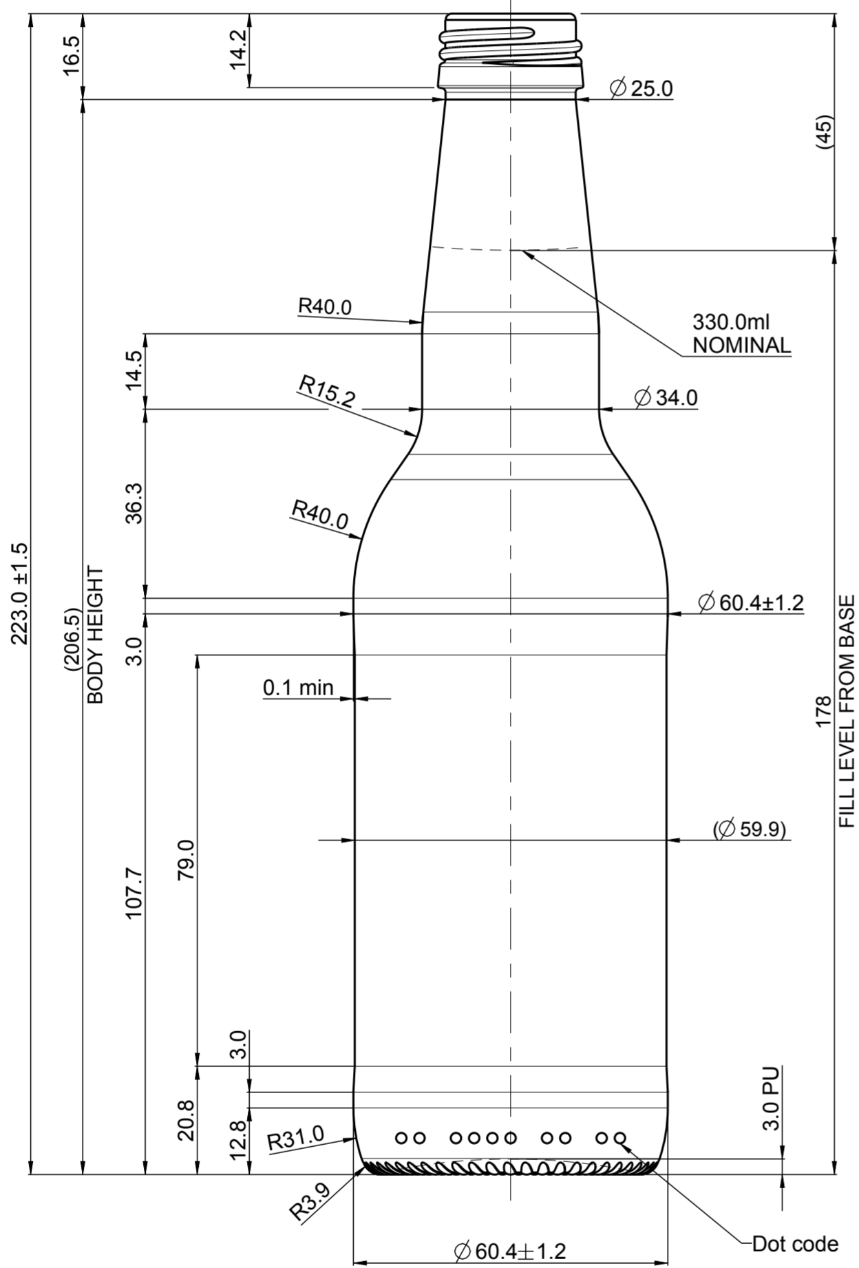
Front view
